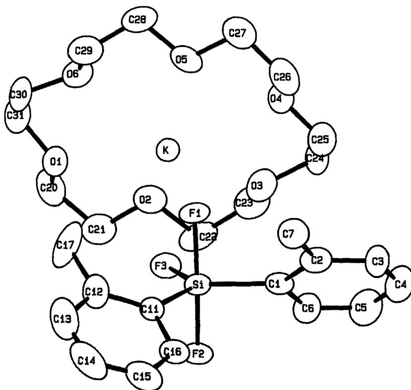
FIGURE 3 ORTEP plot of [o\text{-Tol}_2\text{SiF}_3][\text{K-18-crown-6}] ( 3 ) with thermal ellipsoids at the 30% probability level. Hydrogen atoms are omitted for clarity.
