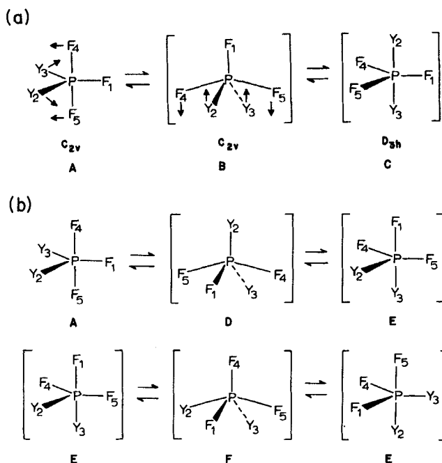
FIGURE 7 Pseudorotational processes for intramolecular exchange in Y_2PF_3 derivatives: (a) simple Berry process; (b) successive Berry processes. Bracketed isomers represent transition states or intermediates.
