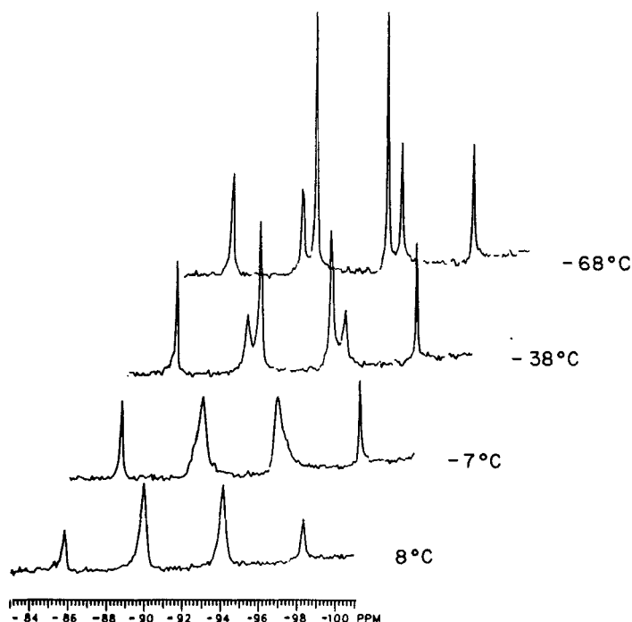
FIGURE 5 Variable-temperature ^{29}Si NMR spectra of [Mes_2SiF_3][K-18-crown-6] showing retention of ^{29}Si - ^{19}F spin-spin coupling from the "stopped" -exchange region, -68^\circ C , to the fast-exchange region, +8^\circ C .
