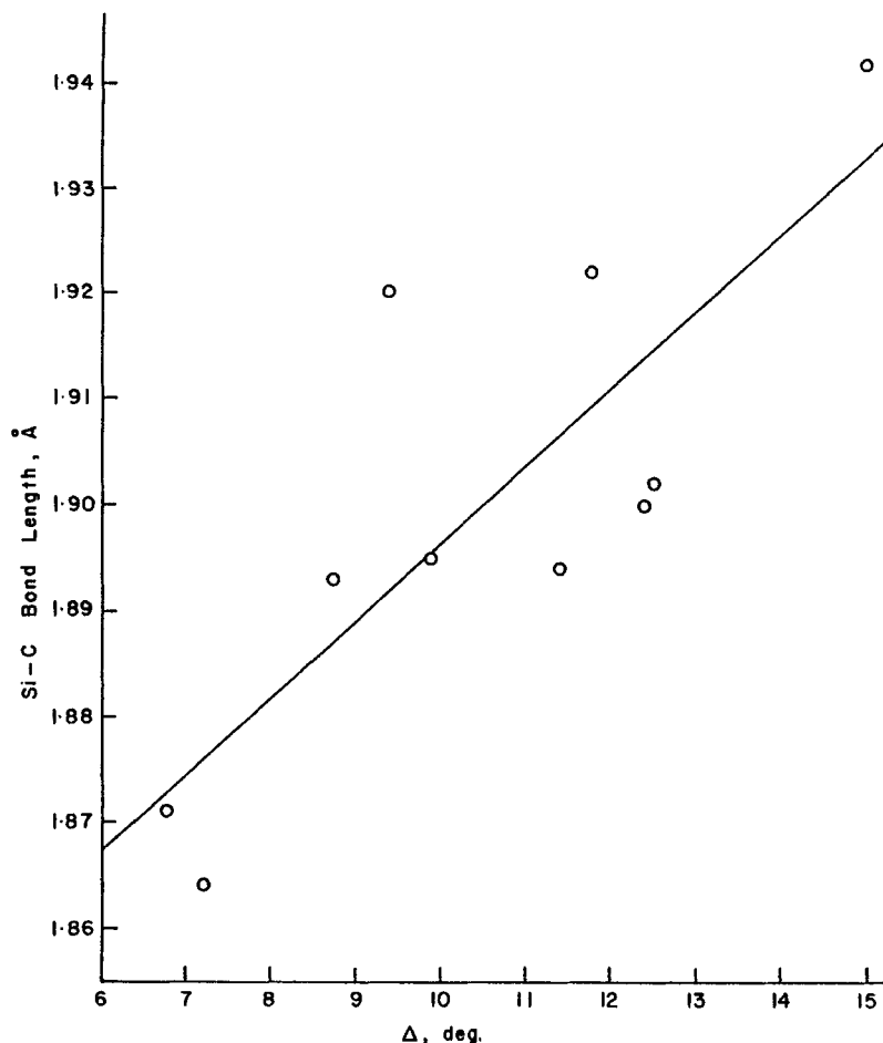
FIGURE 4 Si–C equatorial bond lengths in trigonal-bipyramidal R_nSiF_{5-n}^- anions vs the distortion parameter, \Delta . A least-squares line is shown, (Si-C) = 0.0073\Delta + 1.8236 .
